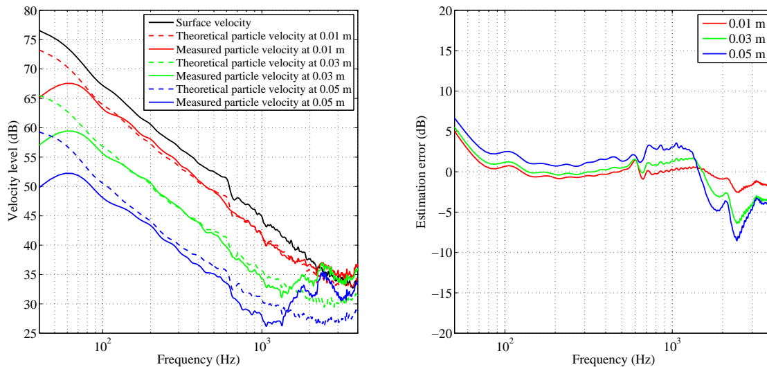
Figure 2 – Comparison of calculated and measured velocity levels using an accelerometer and a particle velocity sensor (left); level difference between calculated and measured surface velocity(right).
