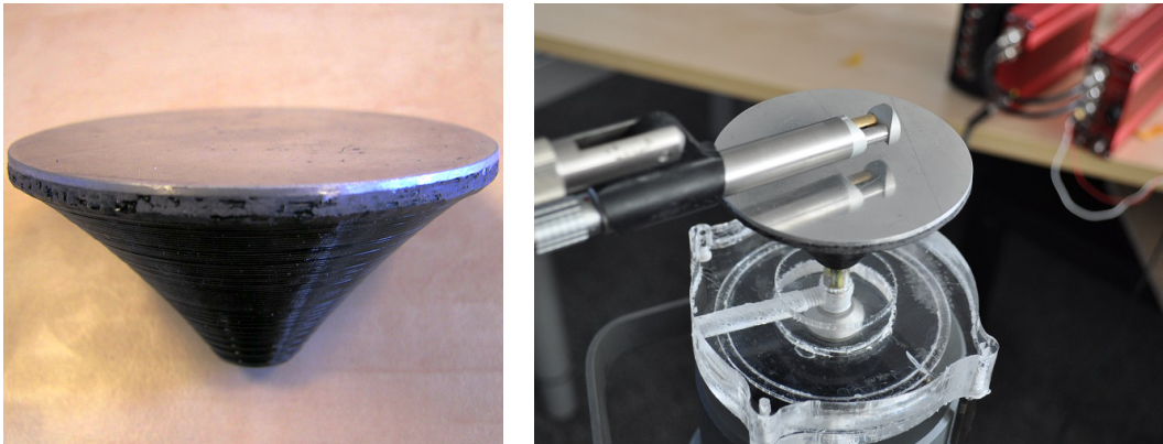
Figure 1 – Piston with aluminium surface (left) and measurement setup (right).
