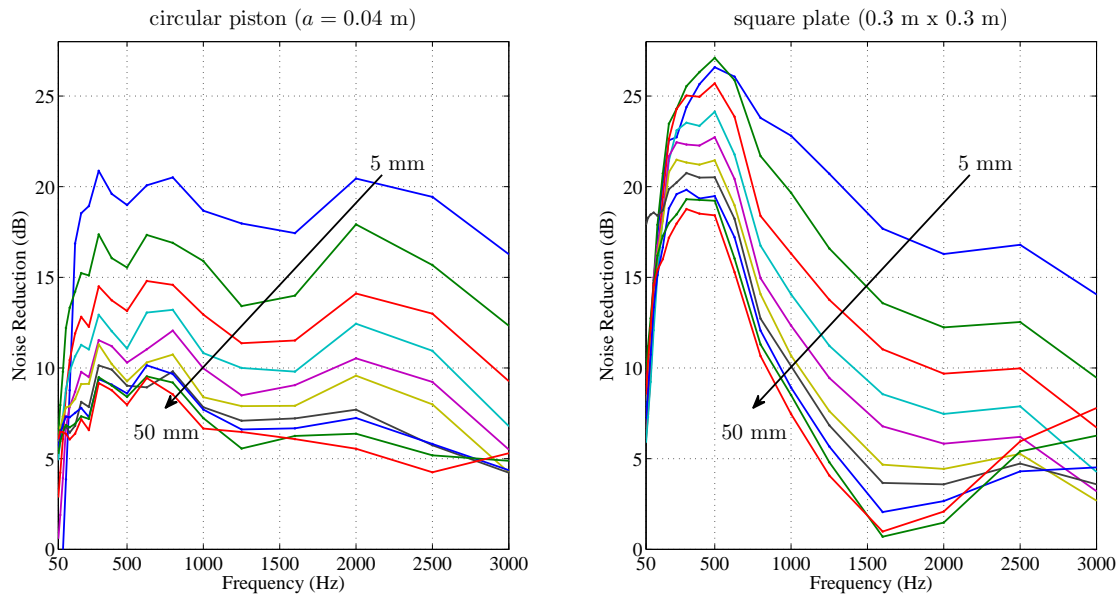
Figure 4 – Noise reduction in front of a rigid circular piston (left) and square wooden plate (right).
