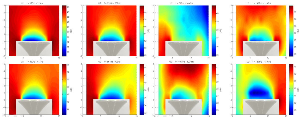
Figure 3 – Acoustic particle velocity perceived around a rigid piston in the presence of background noise.
