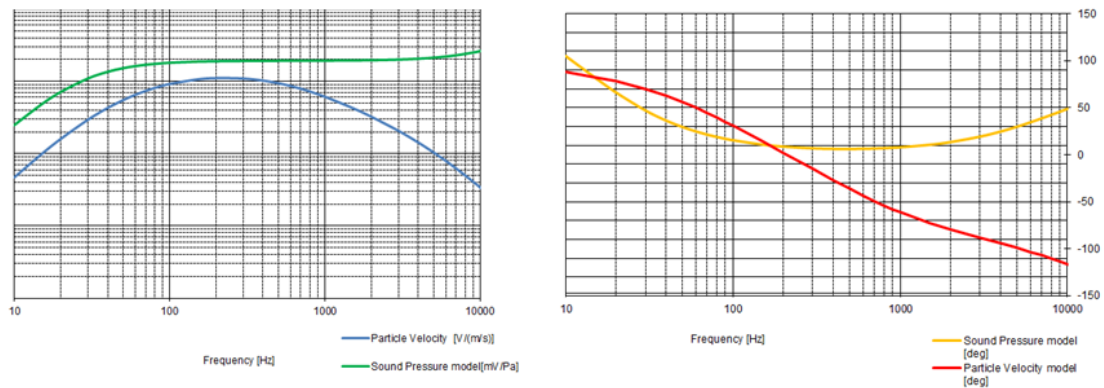
Figure 3. Typical USP regular model
