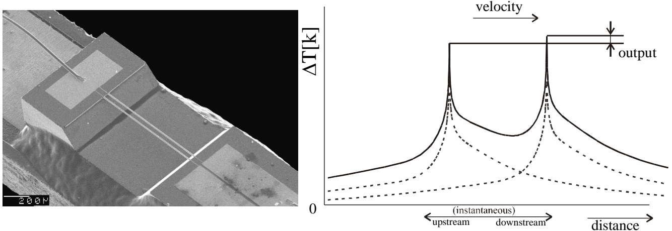
Figure 1. Sensor principle
