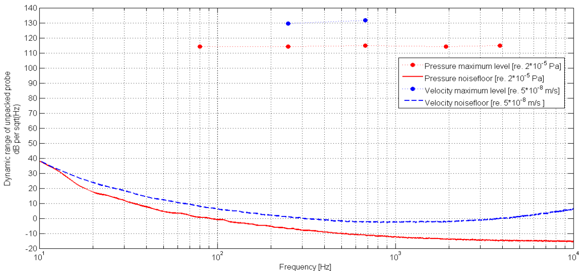
Figure 2. USP regular and MFPA-4 dynamic range
