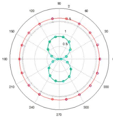
Figure 4: USP regular polar pattern
