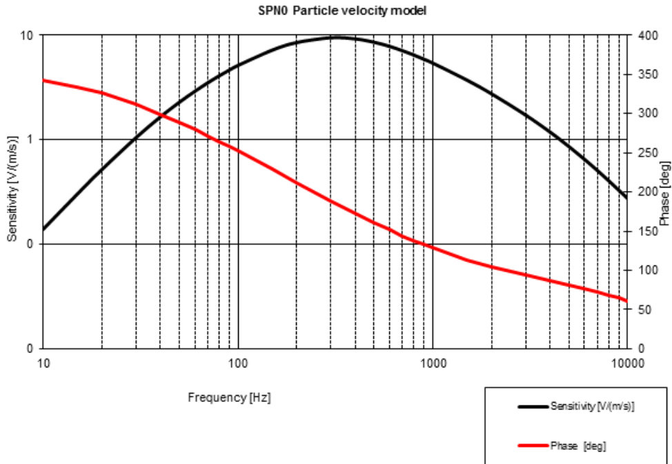
Figure 3. Typical SPN0 Microflown response model
