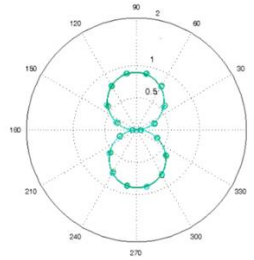
Figure 4: SPN polar pattern
