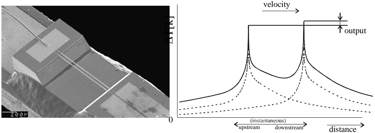
Figure 1. Sensor principle
