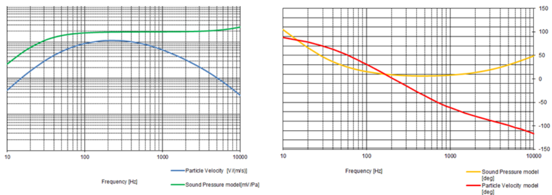
Figure 3. Typical PI model
