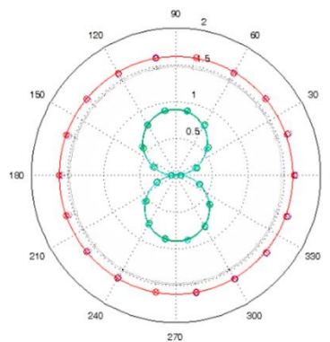
Figure 4: PI polar pattern
