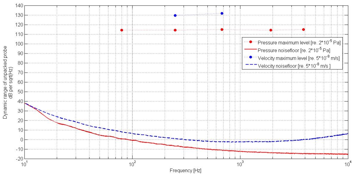
Figure 2. PI probe and MFPA-2 dynamic range
